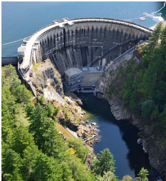
Overview of the entire Cushman Dam
