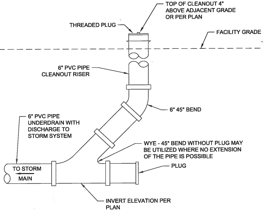
CLEANOUT WITH WYE / BEND SECTION NTS
