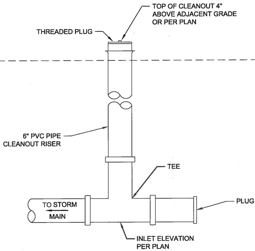
CLEANOUT WITH TEE SECTION NTS
