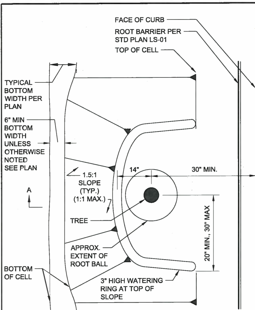
PLAN NTS
