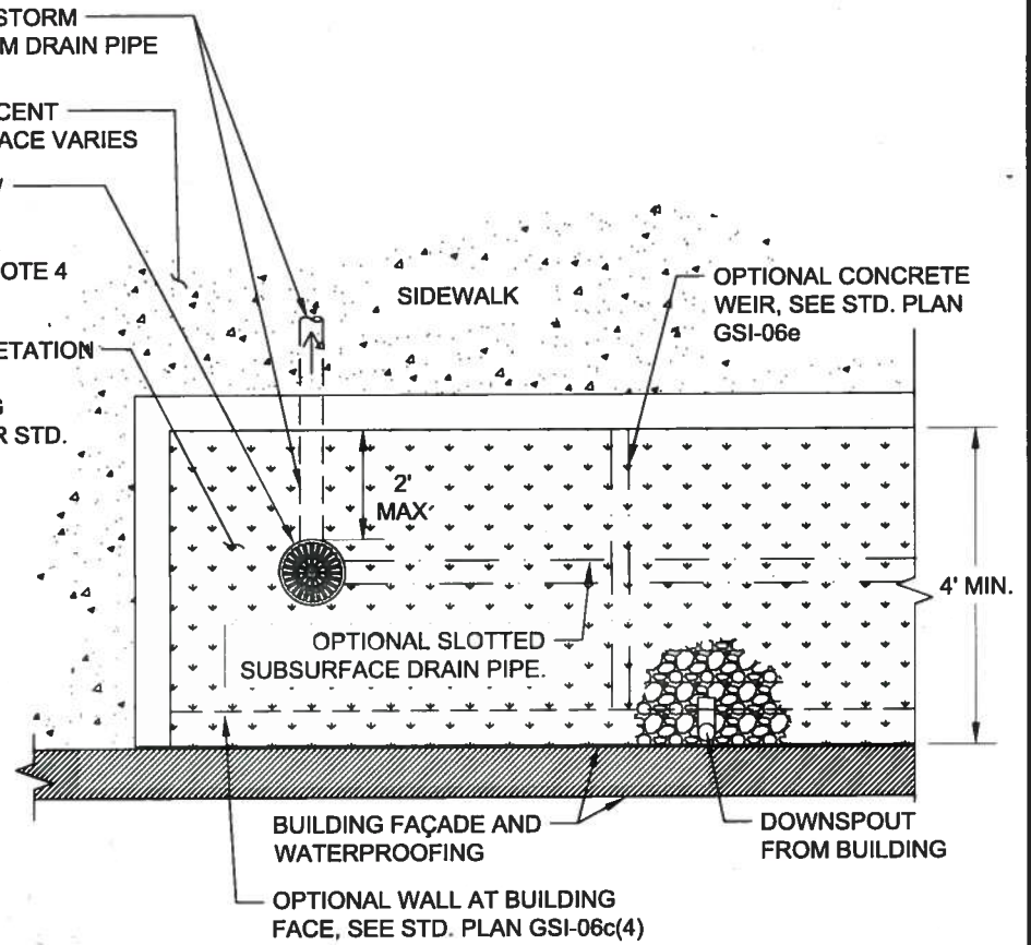
WALLED BIORETENTION ADJACENT TO BUILDING NTS
