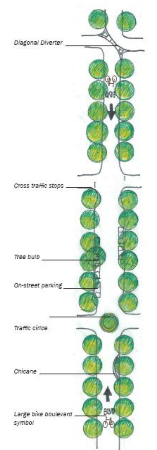
Bicycle Boulevard Treatments Recommended in Tacoma Mixed Use Centers Complete Streets Design Guidelines
