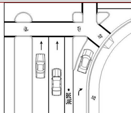
Porkchop refuge island
