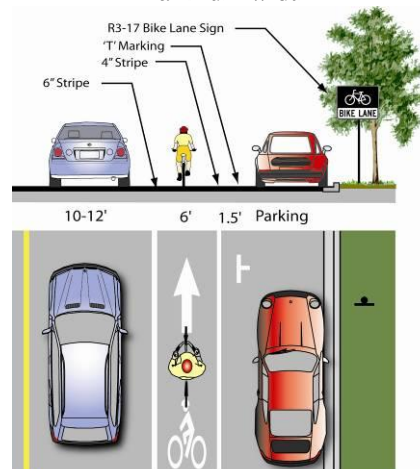
Preferred Design (if space is available)
