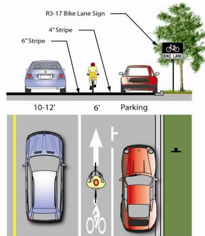
Minimum Design
