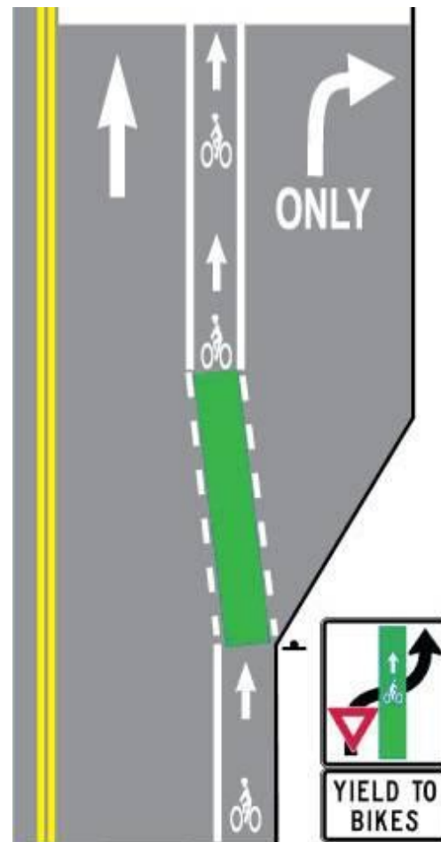
Recommended Design
