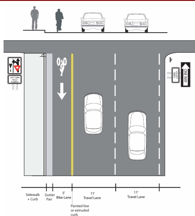
Recommended Design
