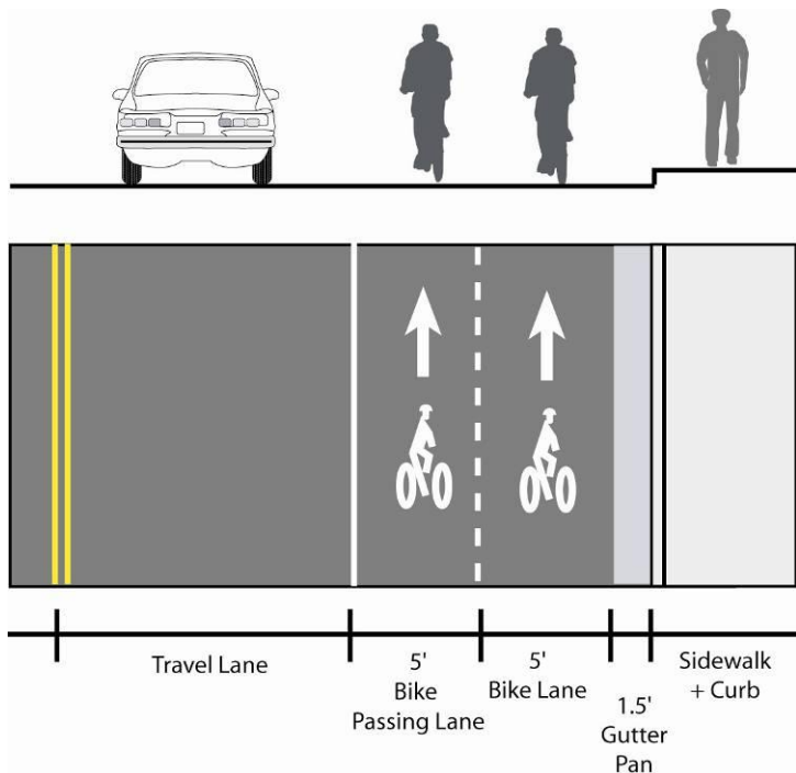
Recommended Design
