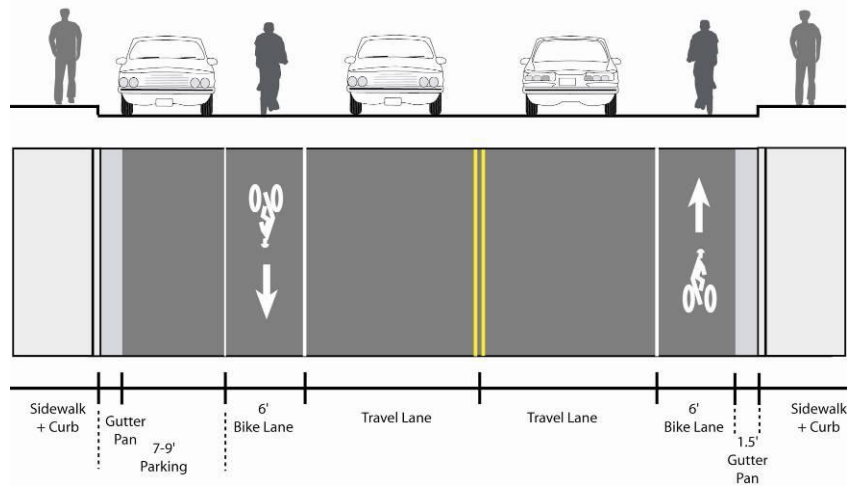
Two Lane Cross-Section with Parking Both Sides
