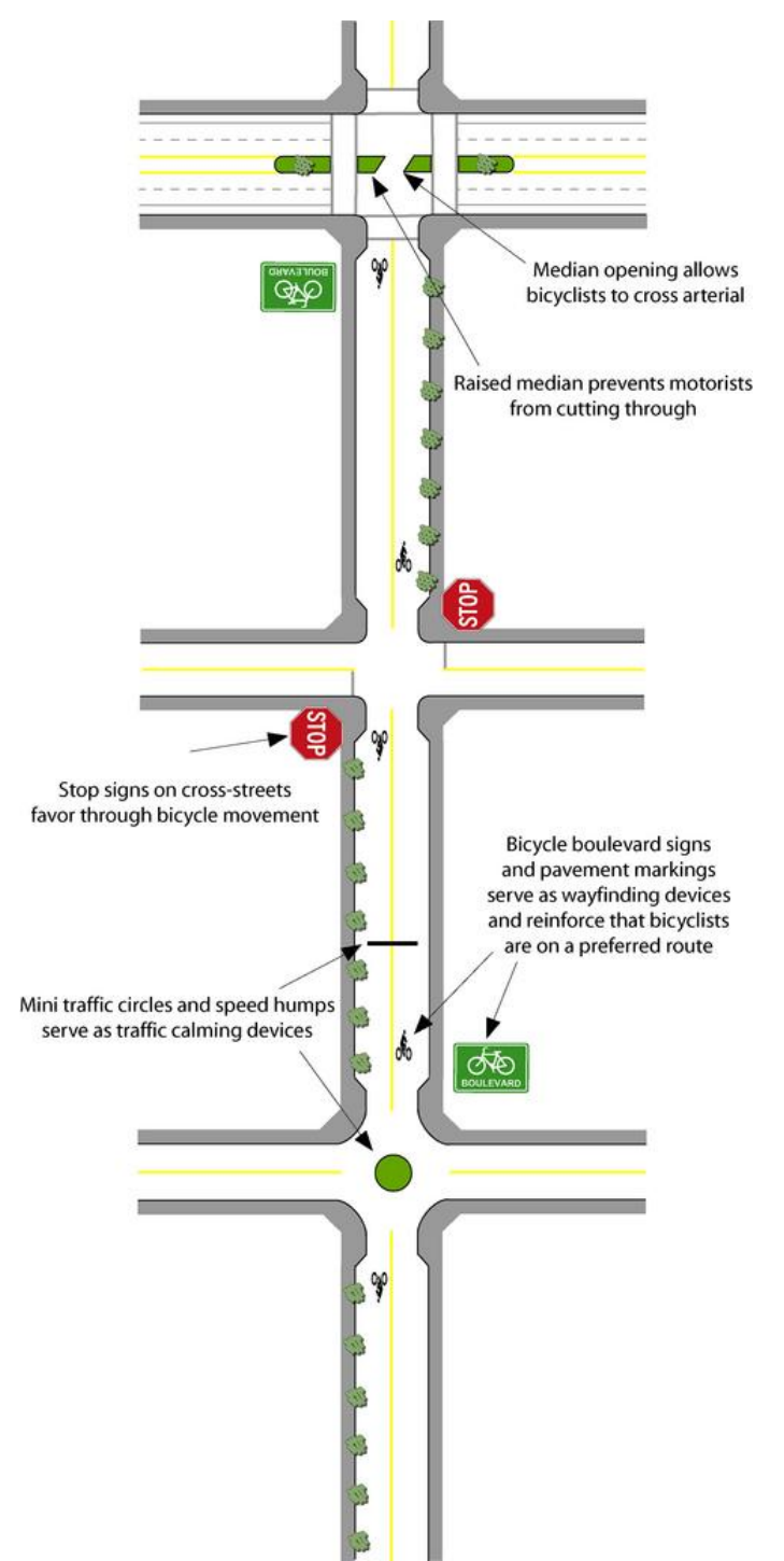
Sample Bicycle Boulevard Treatments
