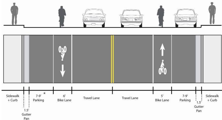
Two Lane Cross-Section with Parking One Side*
