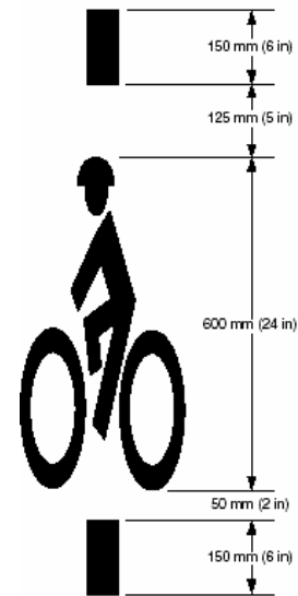
Recommended Design
